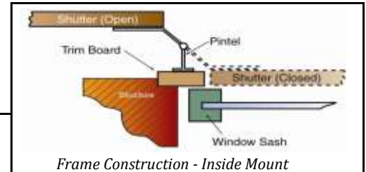
Frame Construction - Inside Mount
